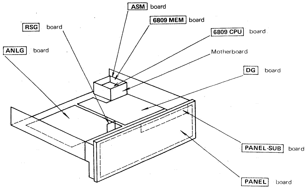
Operation Unit
